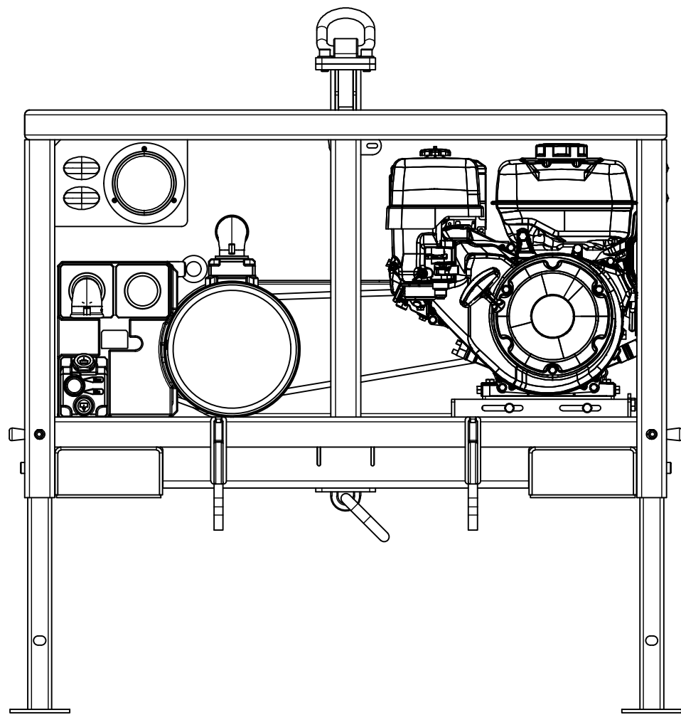
Front view
