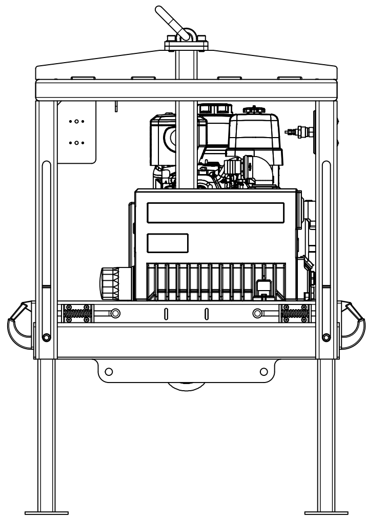
Left view
