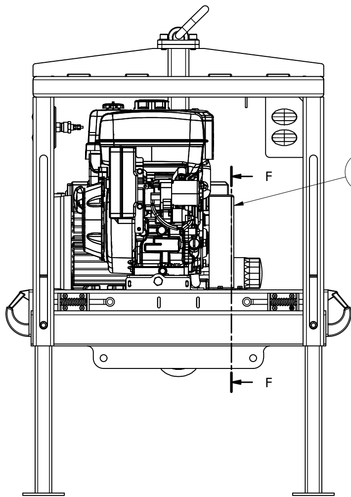
Right view
