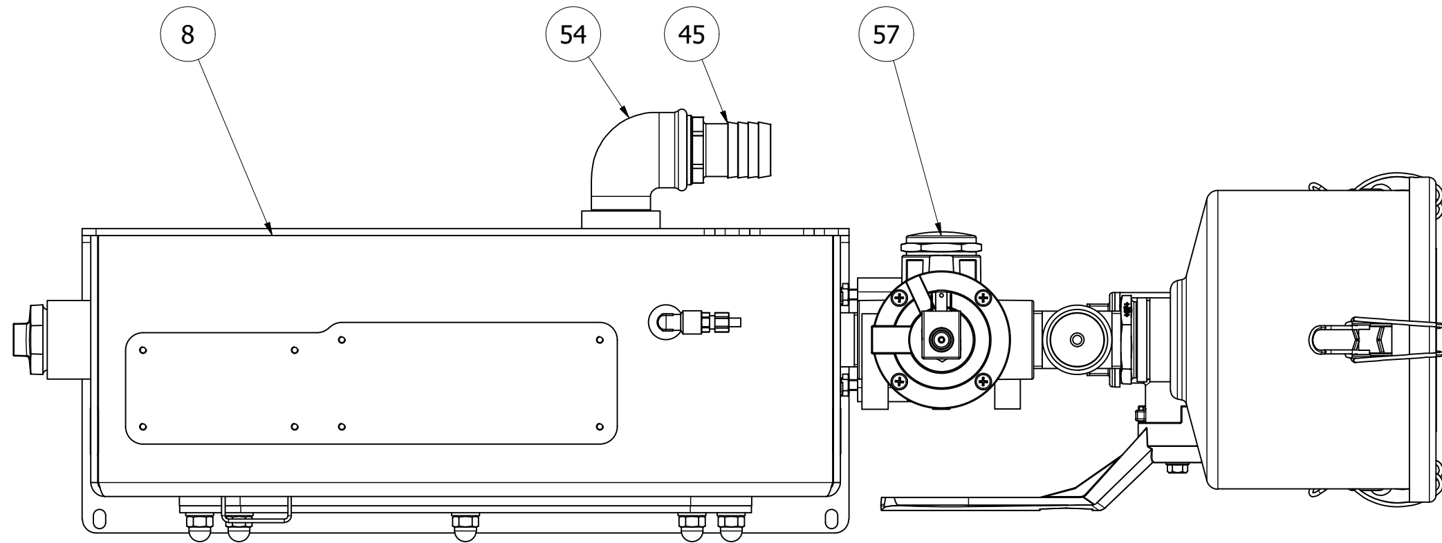
Top view
