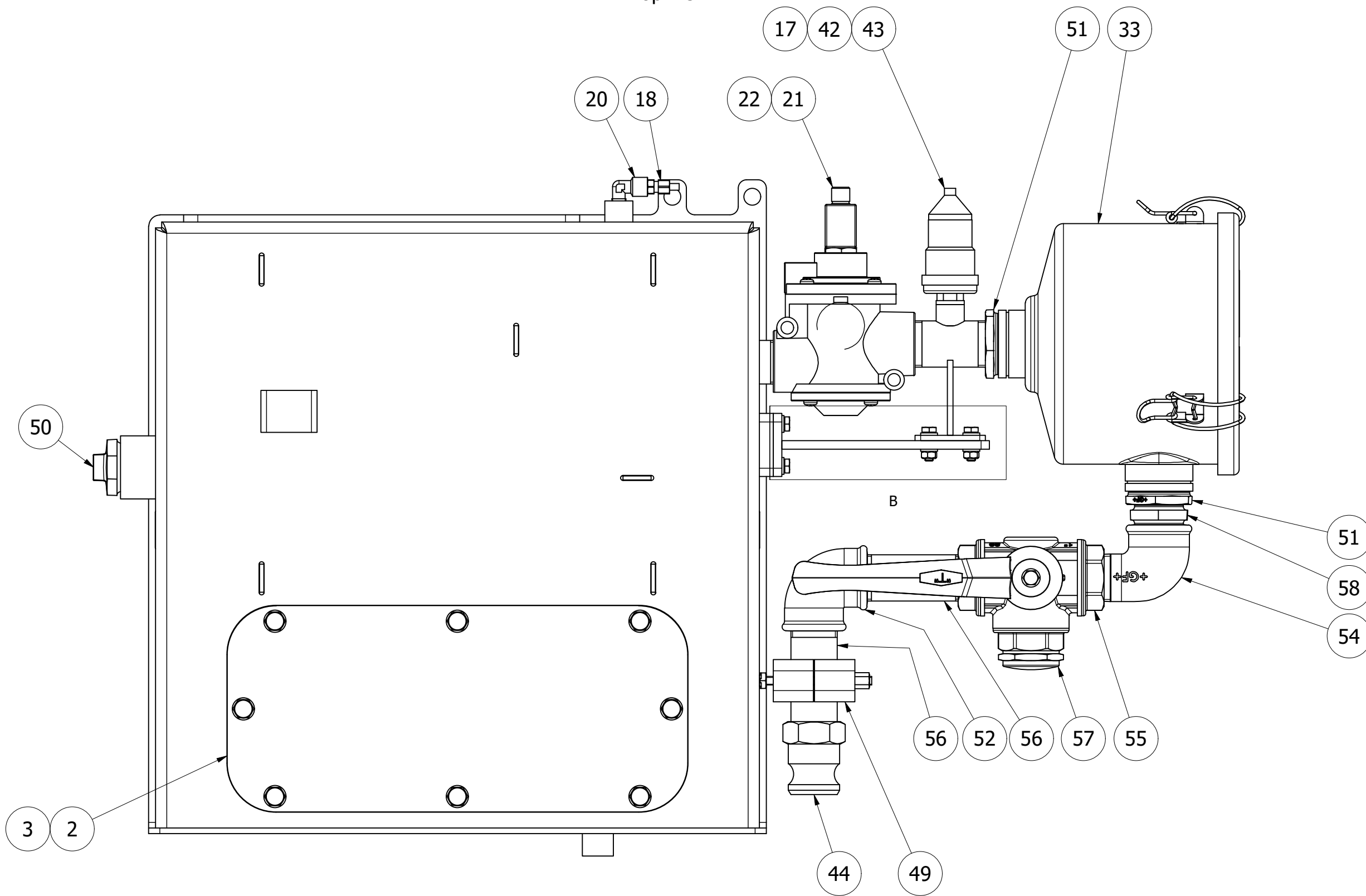
Front view
