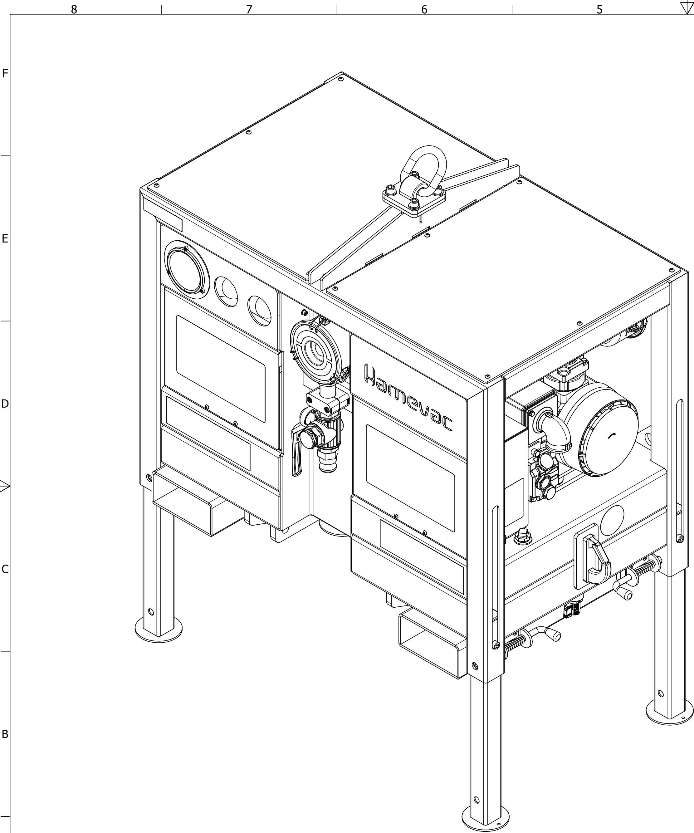
Isometric view
