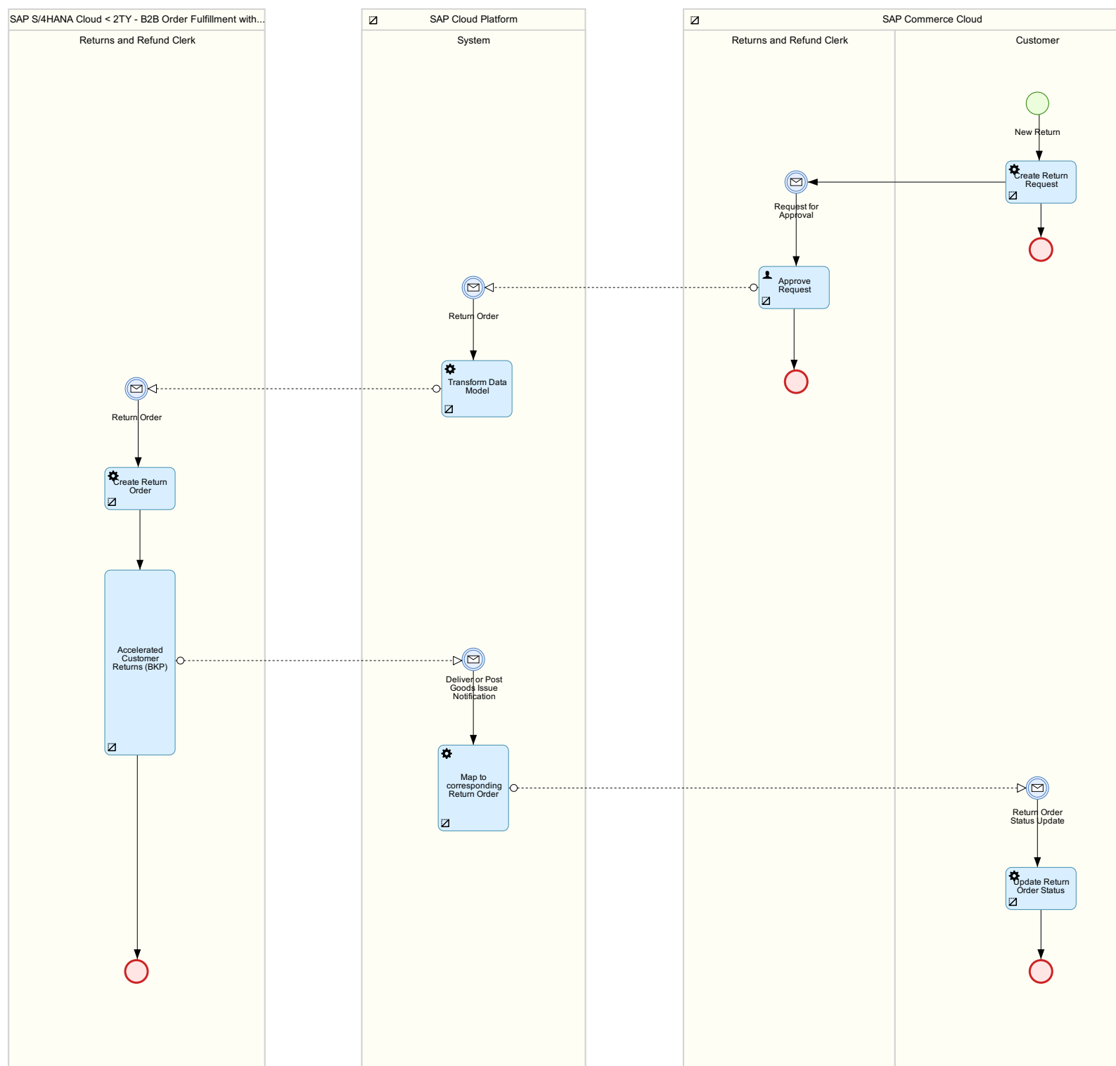
05 - Integration with SAP Commerce Cloud - B2B Asynchronous Order Management - Service Order Processing
